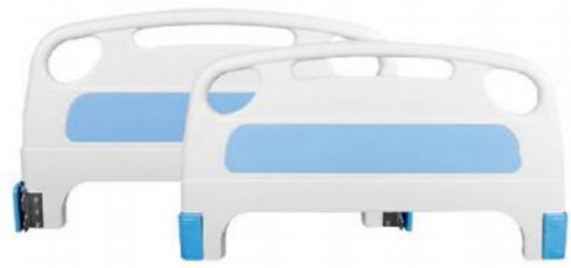
JL10-A HEAD&FOOT BOARD DIMENSION: 950*535MM/950*435MM HOOK DISTANCE: 902MM
